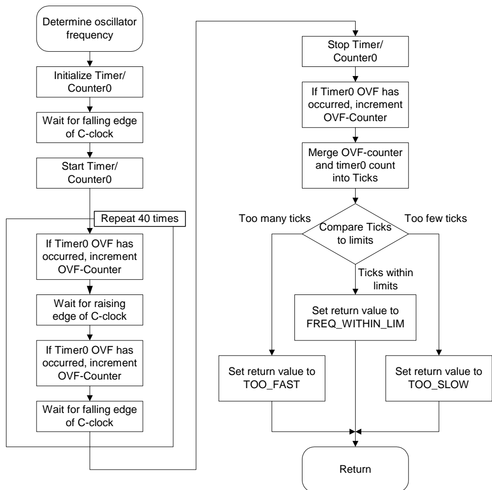
Figure 3. Flowchart of algorithm determining relationship between the C-clock and the internal oscillator frequency.
